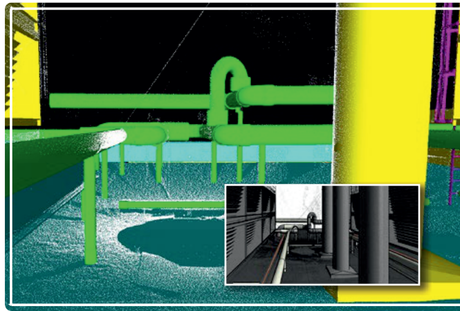
The new workflow of scan to EdgeWise MEP to Revit improved overall efficiency in the hospital MEP modeling project by 70%.
